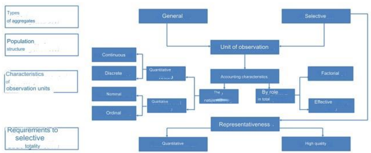
Figure 1.2. Types and structure of the statistical population
