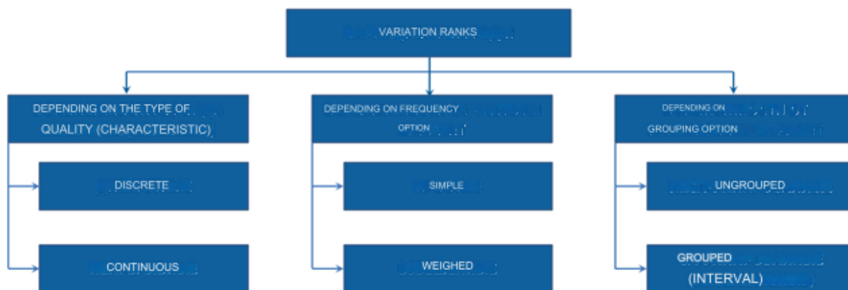
Figure. 2.1. Types of variation series
