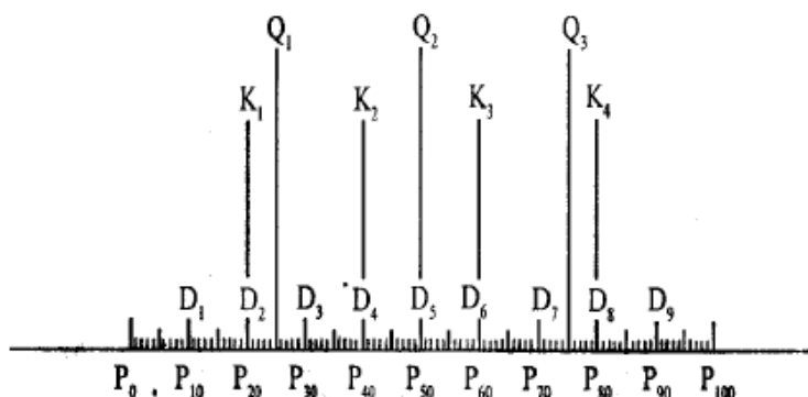
Figure 2.5. Structural characteristics of the variation series
