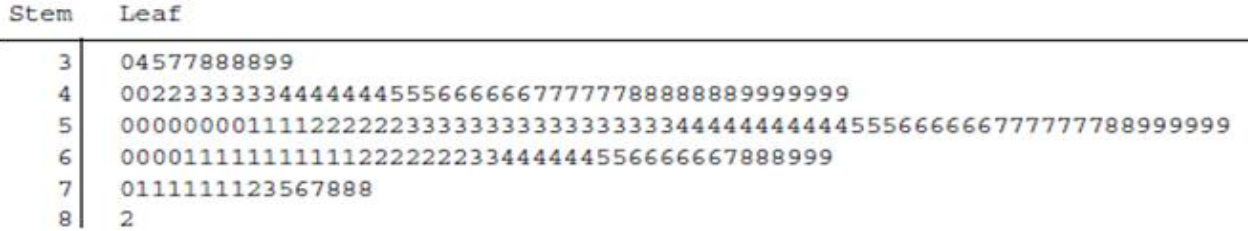
Figure; 2.4. Stem and Leaf Plot
